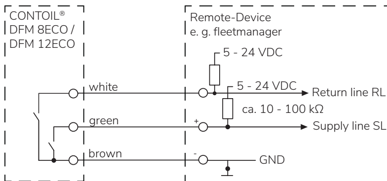
Functional diagram CONTOIL® DFM 8 / 12 ECO pulse specification; passive pulse
