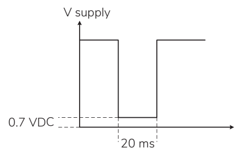
Output signal specification
