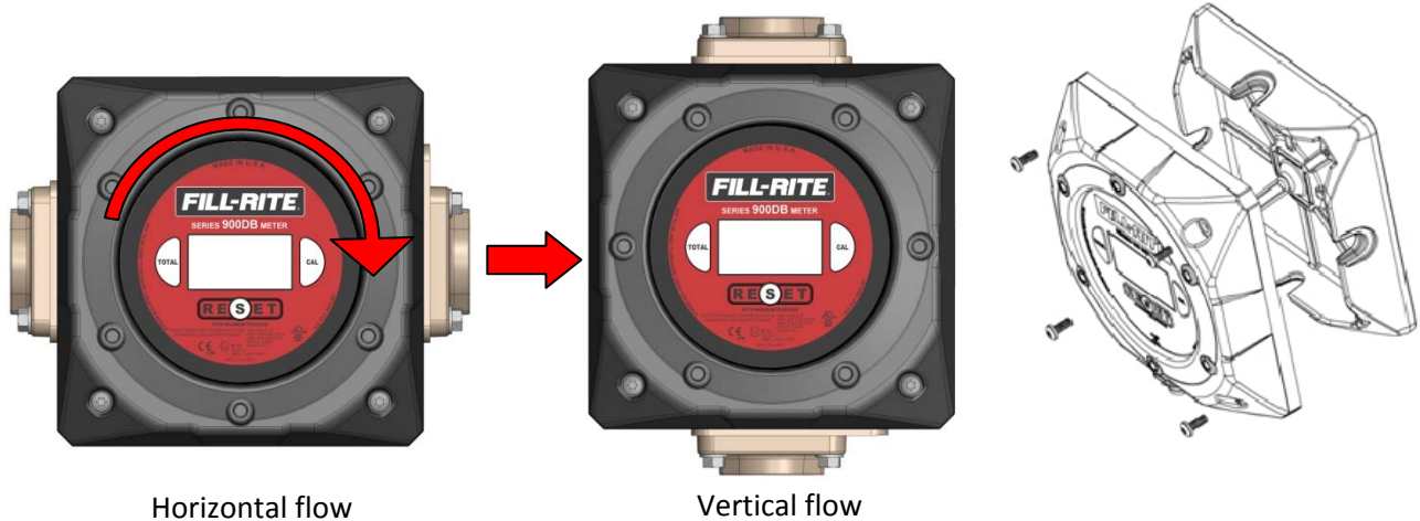
Horizontal flow
